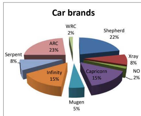
Car brands
