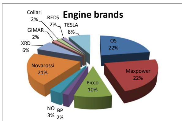
Engine Brands
