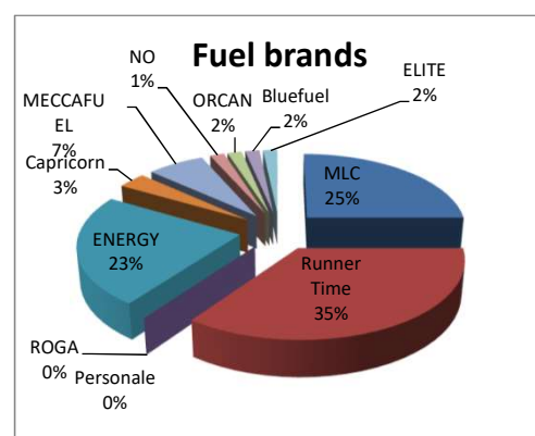
Fuel Brands
